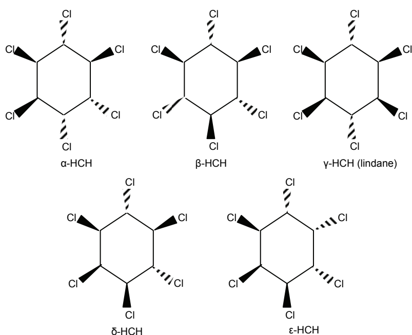
Figure 2.2. The chemical structures of the HCH-isomers.
