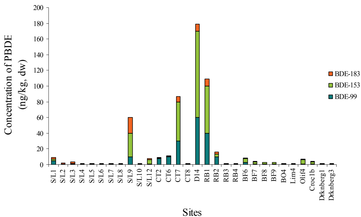
Figure 4.8 The contribution of BDE-183, -153 and -99 towards the Σ-PBDE measured at each site.
