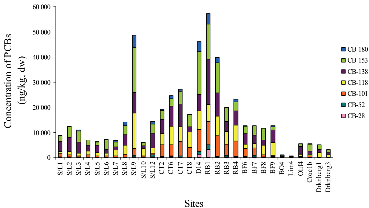
Figure 4.7 The contribution of the seven PCB congeners to the ΣPCBs measured at each site.
