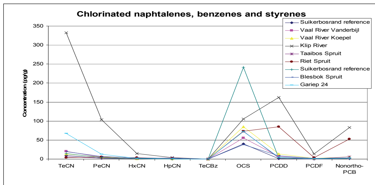
Figure 2. Chlorinated naphthalene, benzene and styrene profile
